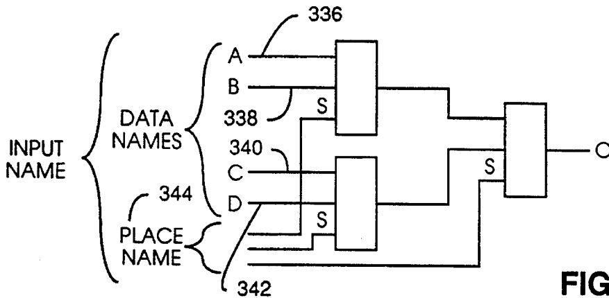
CASCADED SELECTOR TREE
