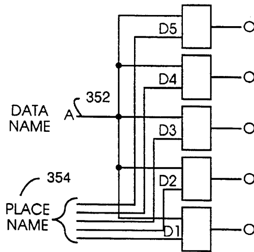
DISTRIBUTOR GROUP
