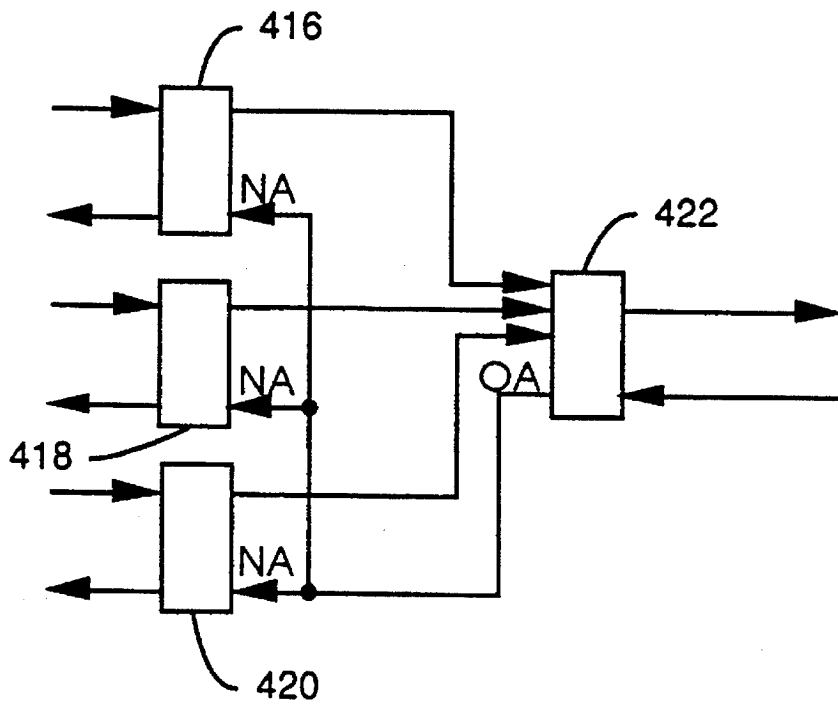
FAN IN CONFIGURATION OF BOUNDARY ELEMENTS
