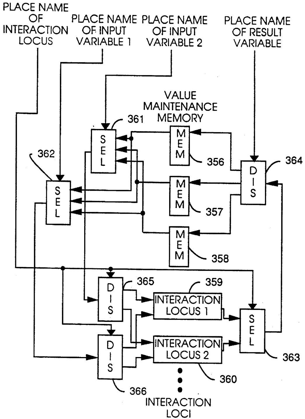
EXPRESSION WITH CONFIGURABLE ASSOCIATION RELATIONSHIPS
