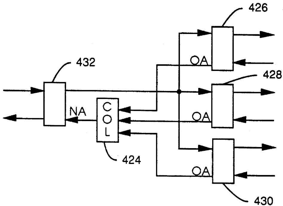
FAN OUT CONFIGURATION OF BOUNDARY ELEMENTS
