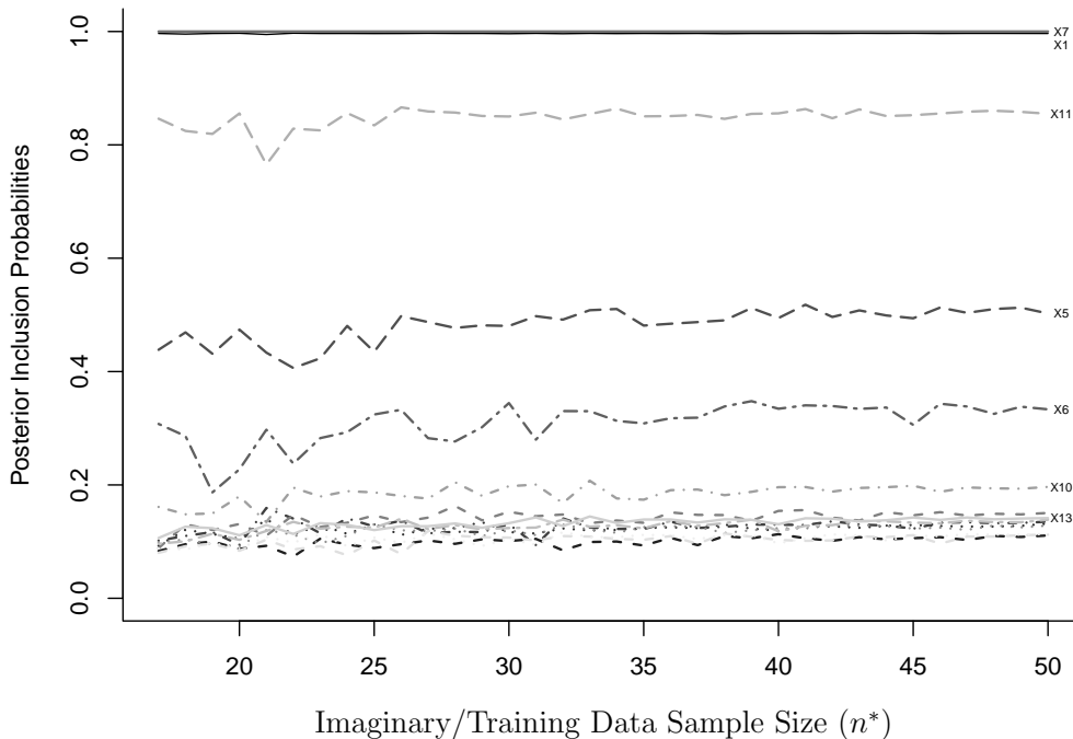
Figure 1: Posterior marginal inclusion probabilities, for n^* values from 17 to n = 50 , with the Z-PEP prior methodology, in the simulated example of Section 5.1.
