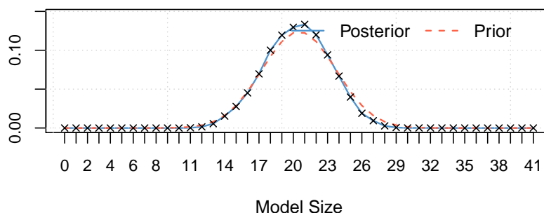
Posterior Model Size Distribution Mean: 20.338
