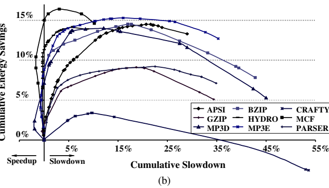
Figure 4. Energy-delay tradeoff curve for BZIP (a) and for all the applications (b).
