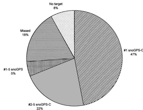
FIGURE 2. Fraction of previously known H/ACA RNAs detected by snoGPS and snoGPS-C. An H/ACA RNA was considered “detected” if it was among the five highest scoring hmr20 sequences for at least one rRNA or snRNA \Psi . The “No target” sequences included H/ACA RNAs with no predicted target as well as those whose associated \Psi was only experimentally located subsequent to these studies. The “#1–5 snoGPS” sequences include those that ranked among the five snoGPS-highest-scoring human sequences for at least one target, but that were not detected using snoGPS-C composite scores. “Missed” sequences did not rank among the top five for any target either for snoGPS or snoGPS-C.
