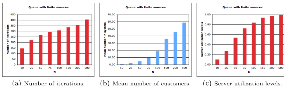
Fig. 4. Behavior of the method for a multi-server queue with c = 8 servers and service time distribution Dist. IV ( cv = 8 , cf. Table 1) as a function of the number of sources N .
