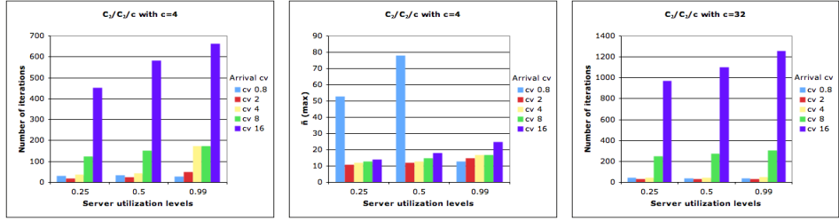
(a) Number of iterations with 4 servers. (b) Maximum value of \tilde{n}^i with 4 servers. (c) Number of iterations with 32 servers.
