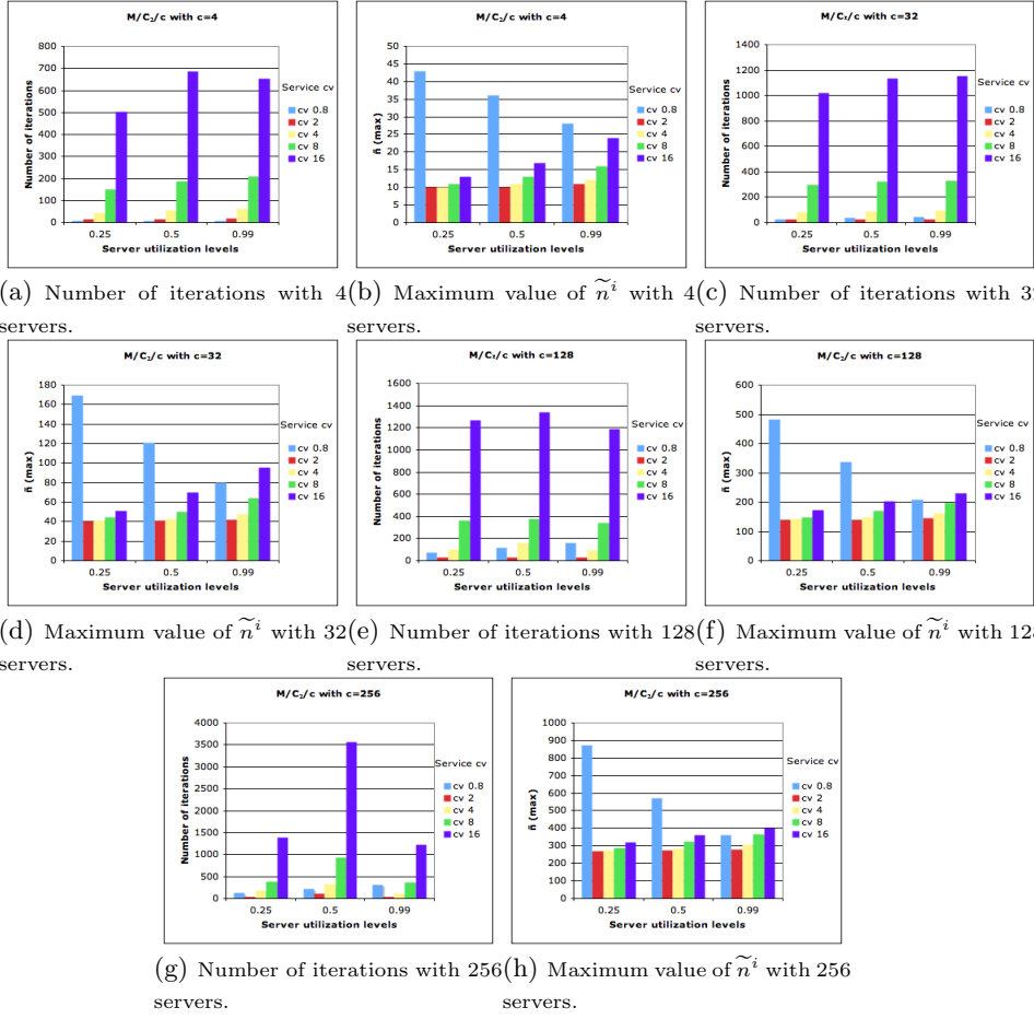
Fig. 2. Behavior of the method for a multi-server queue for service time distributions from Table 1 as a function of the number of servers c and the server utilization level.
