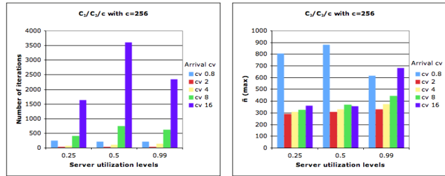
(g) Number of iterations with 256 servers. (h) Maximum value of \tilde{n}^i with 256 servers.
